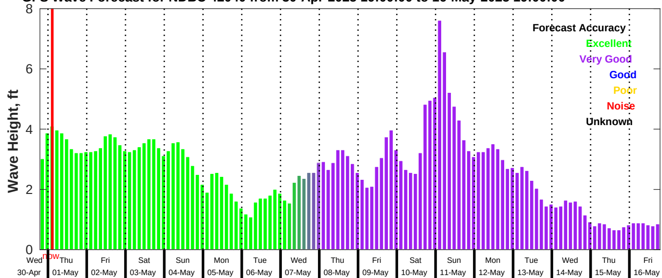
GFS Wave Forecast for NDBC 42040 from 30-Apr-2025 19:00:00 to 16-May-2025 19:00:00
