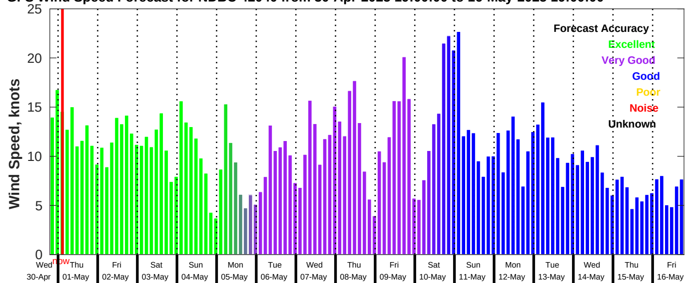
GFS Wind Speed Forecast for NDBC 42040 from 30-Apr-2025 19:00:00 to 16-May-2025 19:00:00
