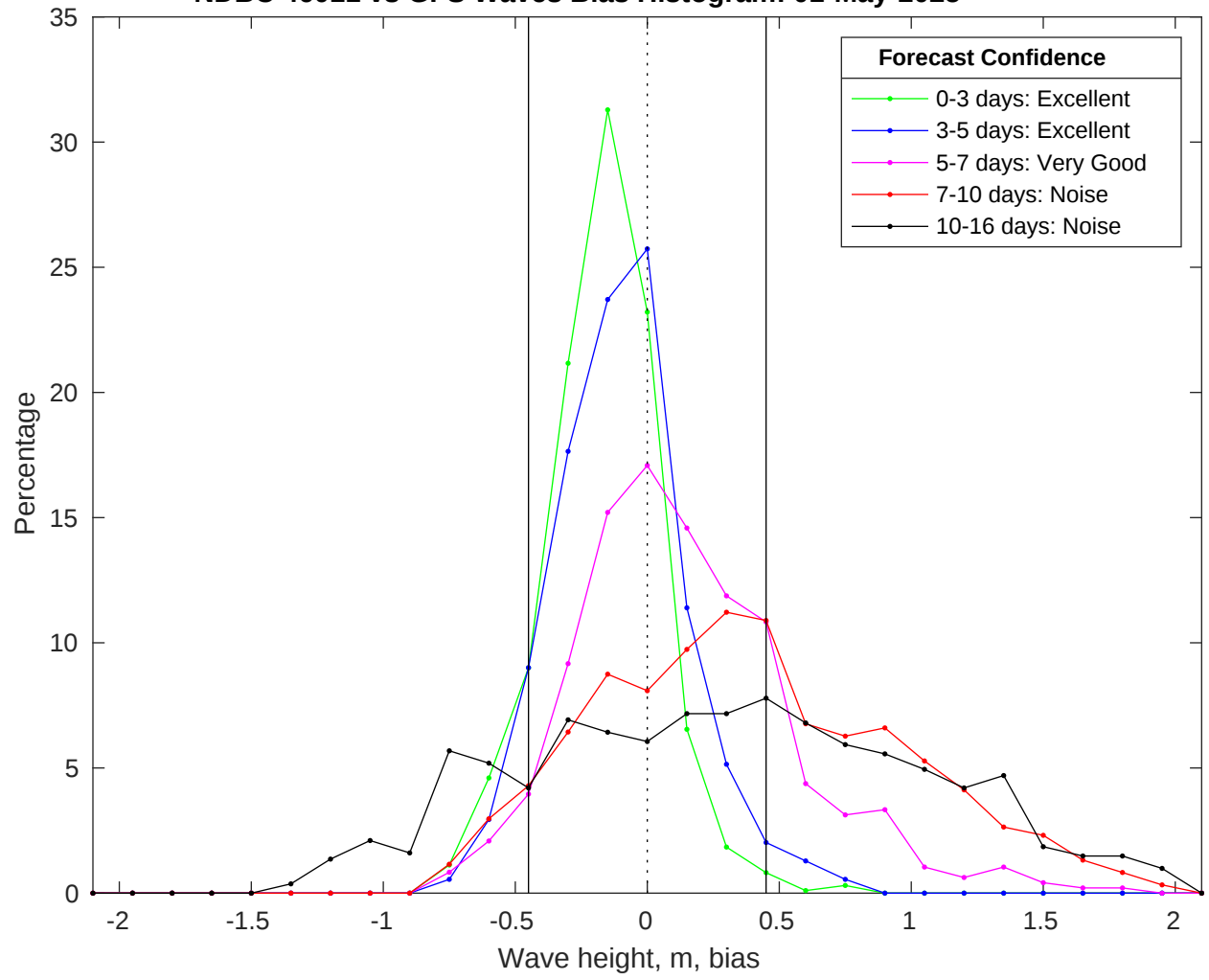
NDBC 46011 vs GFS Waves Bias Histogram: 01-May-2025
