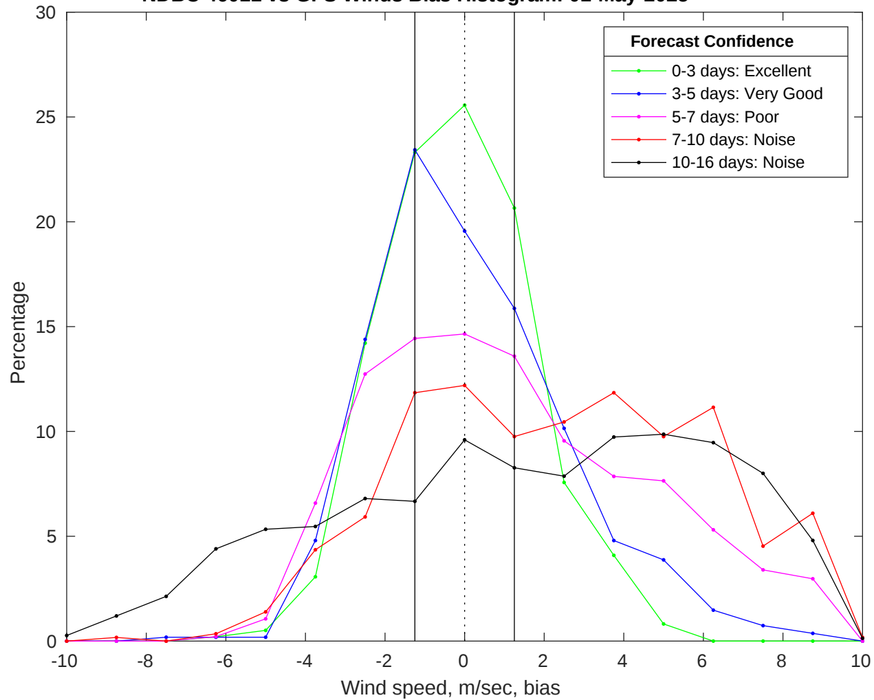
NDBC 46011 vs GFS Winds Bias Histogram: 01-May-2025
