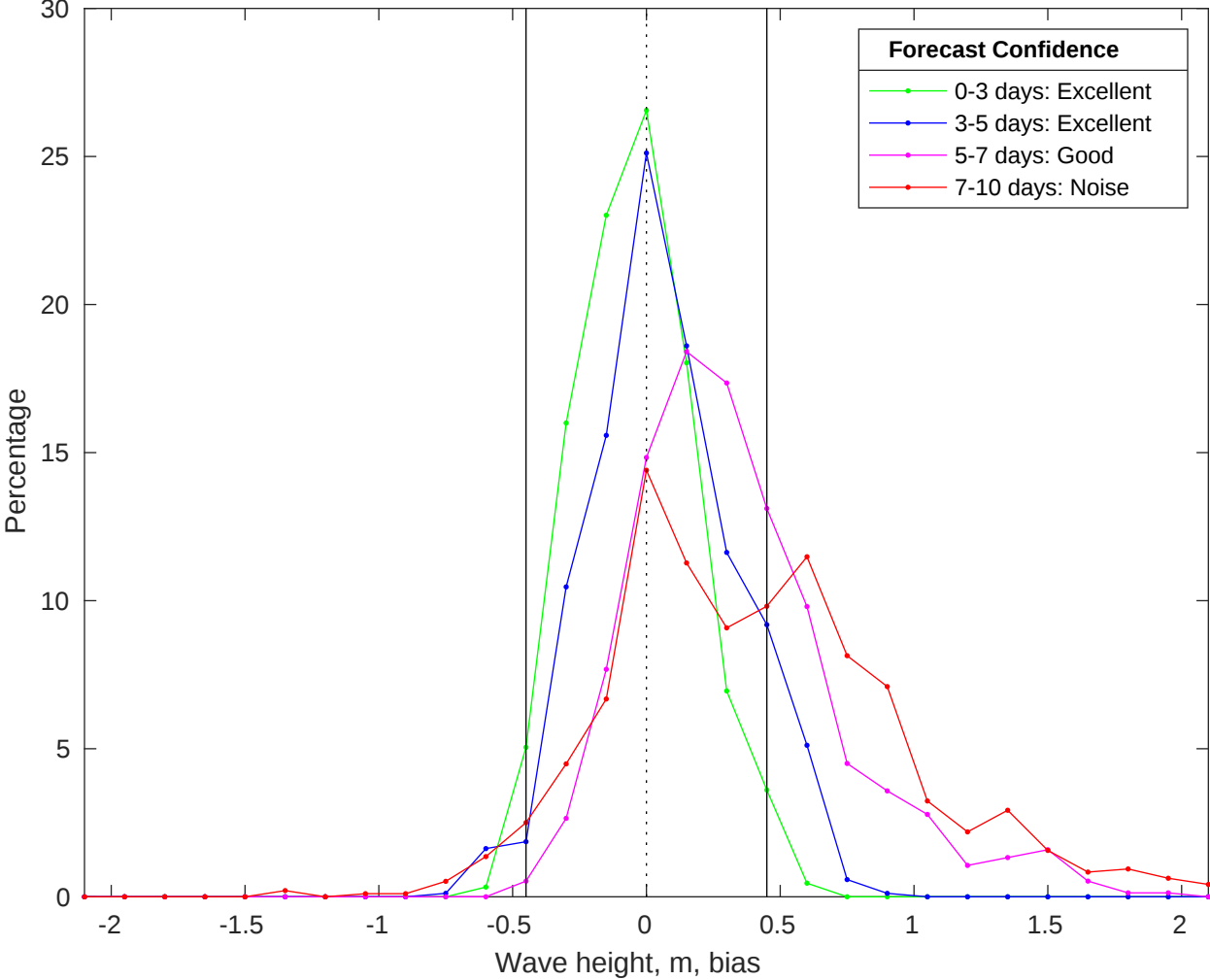
NDBC 46028 vs CMEMS Waves Bias Histogram: 01-May-2025
