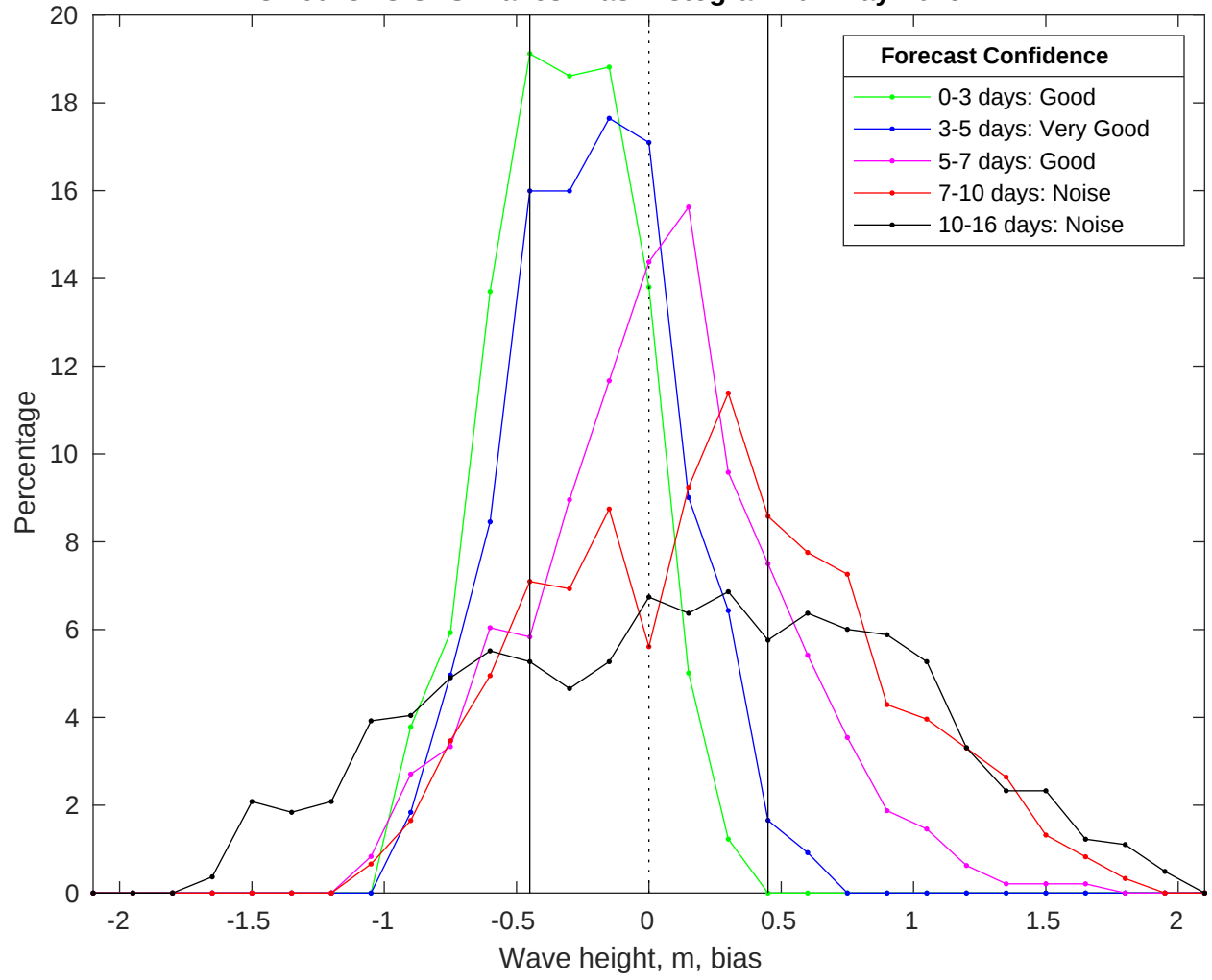
NDBC 46028 vs GFS Waves Bias Histogram: 01-May-2025
