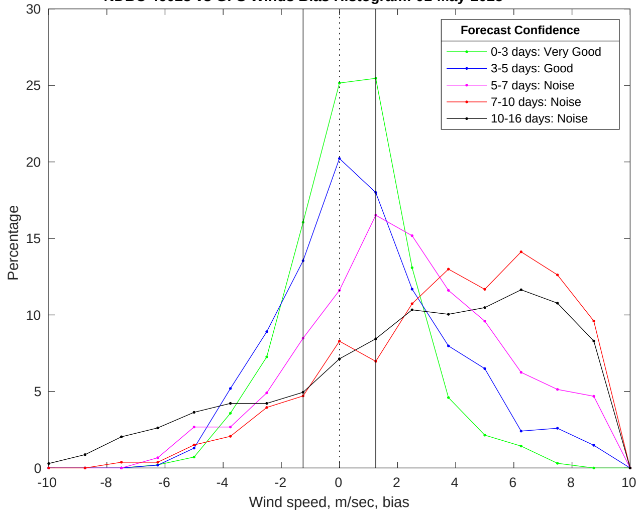
NDBC 46028 vs GFS Winds Bias Histogram: 01-May-2025
