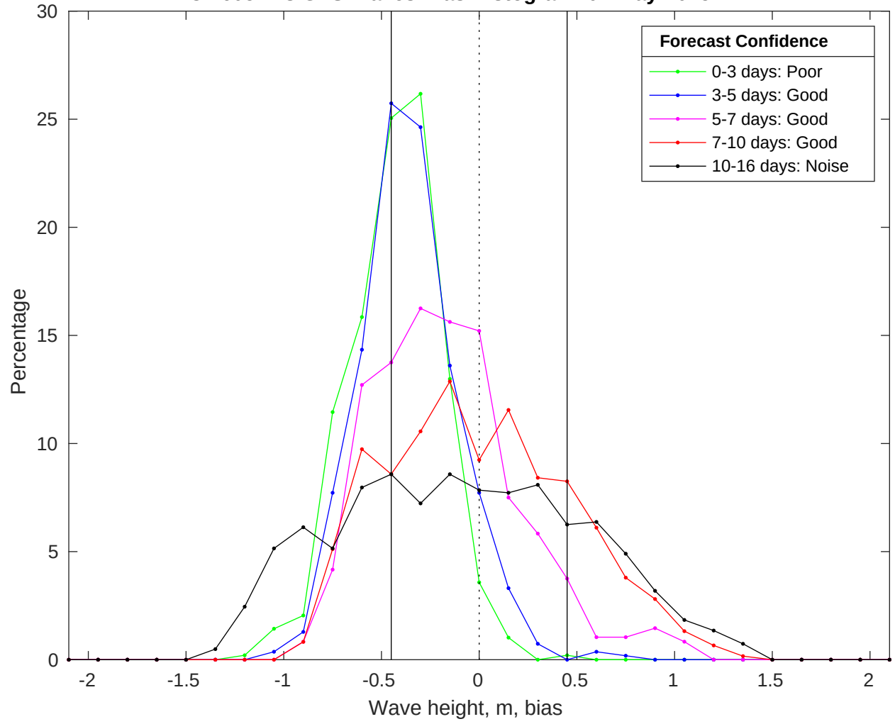
NDBC 46054 vs GFS Waves Bias Histogram: 01-May-2025
