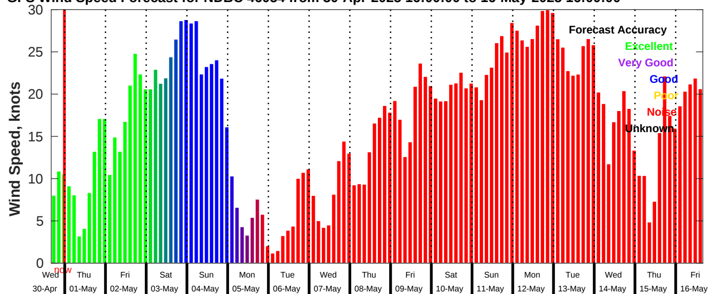
GFS Wind Speed Forecast for NDBC 46054 from 30-Apr-2025 16:00:00 to 16-May-2025 16:00:00
