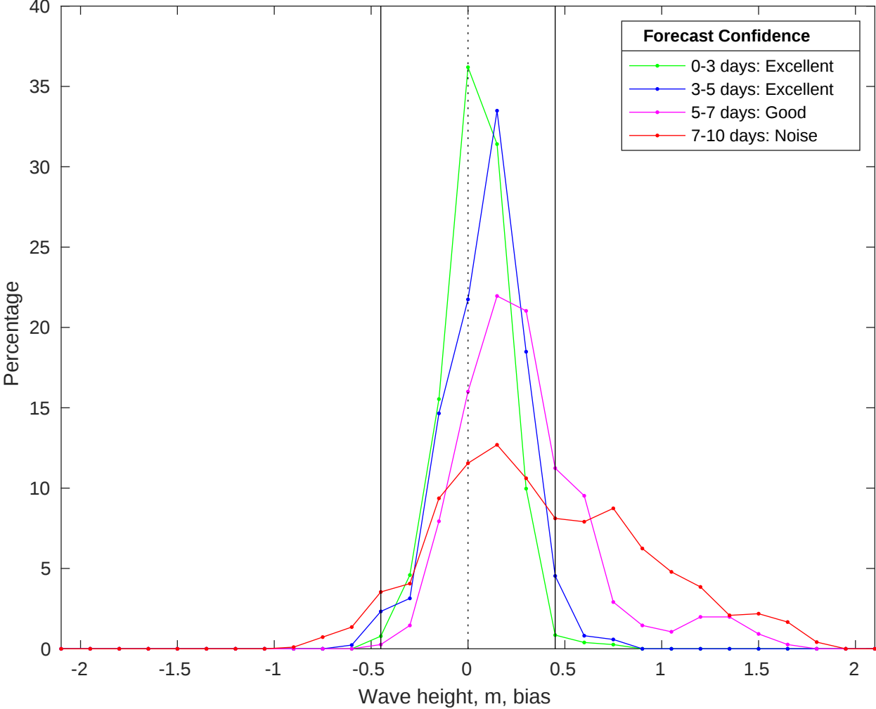
NDBC 46069 vs CMEMS Waves Bias Histogram: 01-May-2025
