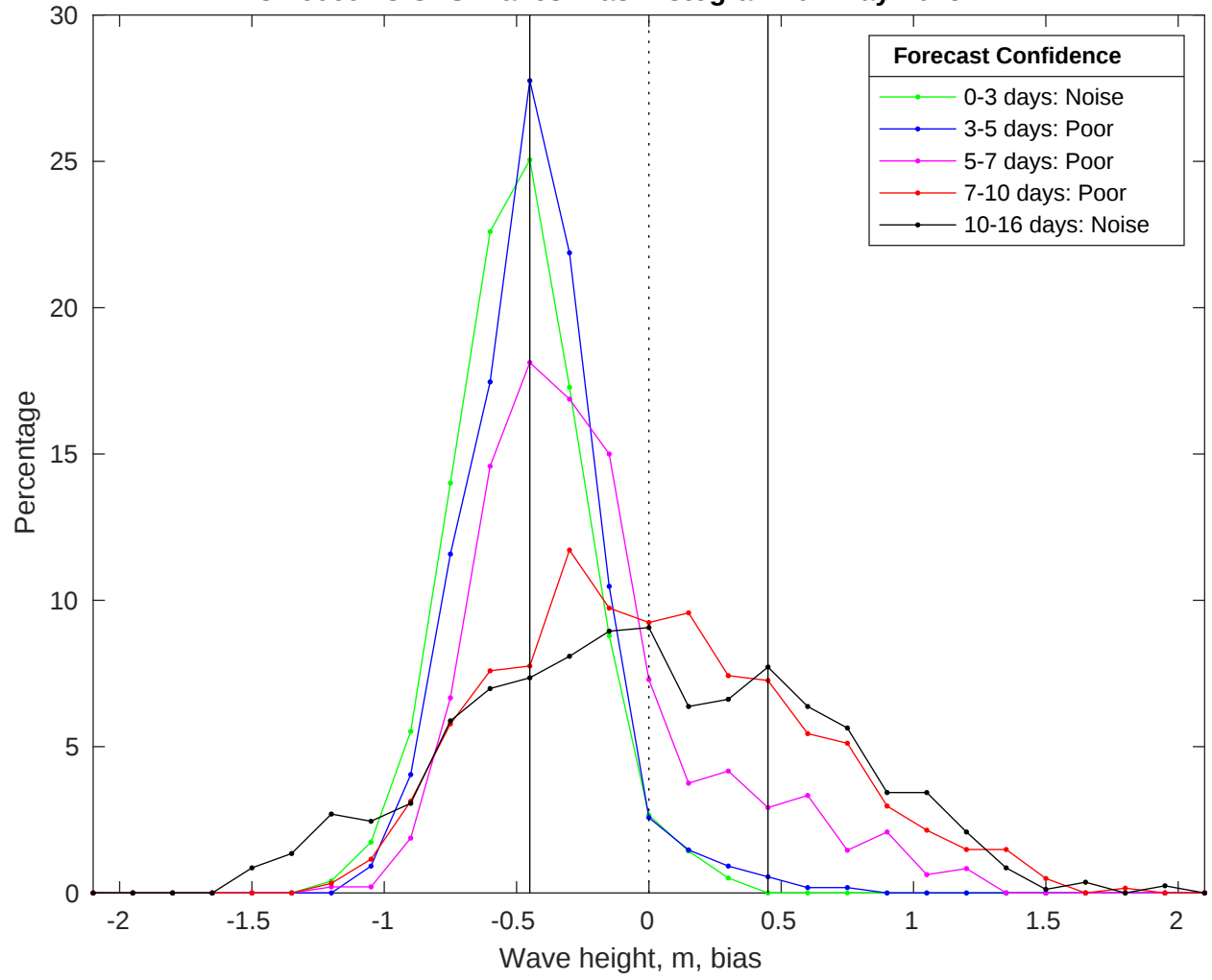
NDBC 46069 vs GFS Waves Bias Histogram: 01-May-2025
