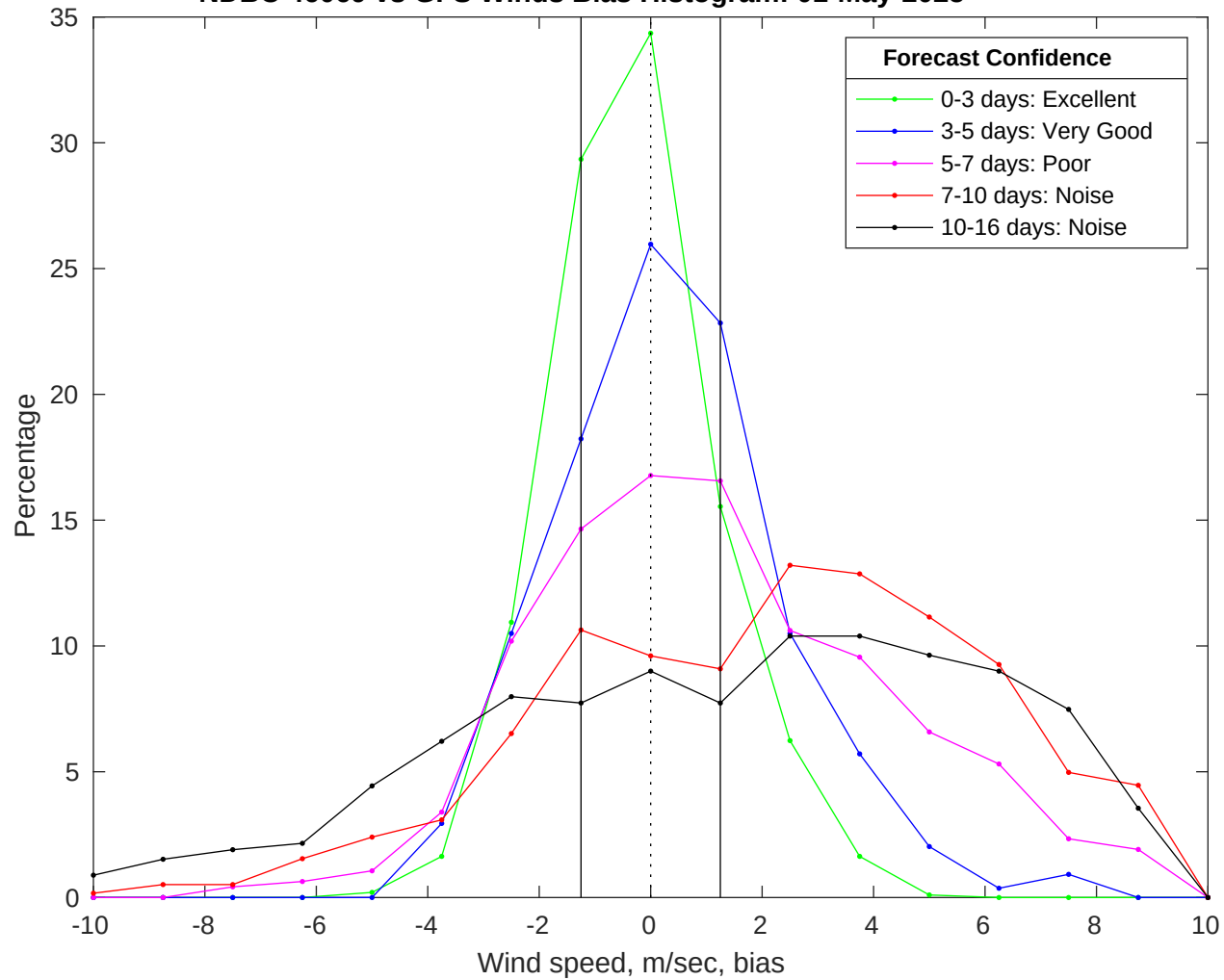
NDBC 46069 vs GFS Winds Bias Histogram: 01-May-2025
