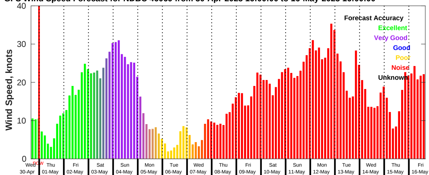
GFS Wind Speed Forecast for NDBC 46069 from 30-Apr-2025 16:00:00 to 16-May-2025 16:00:00
