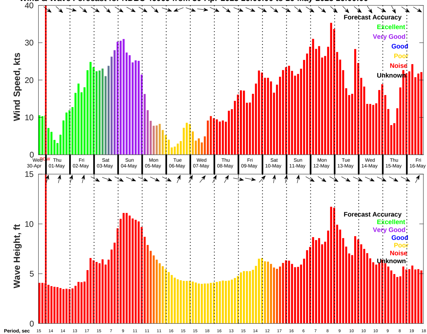
Wind & Wave Forecast for NDBC 46069 from 30-Apr-2025 16:00:00 to 16-May-2025 16:00:00
