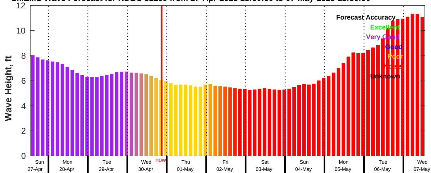
CMEMS Wave Forecast for NDBC 51209 from 27-Apr-2025 13:00:00 to 07-May-2025 13:00:00
