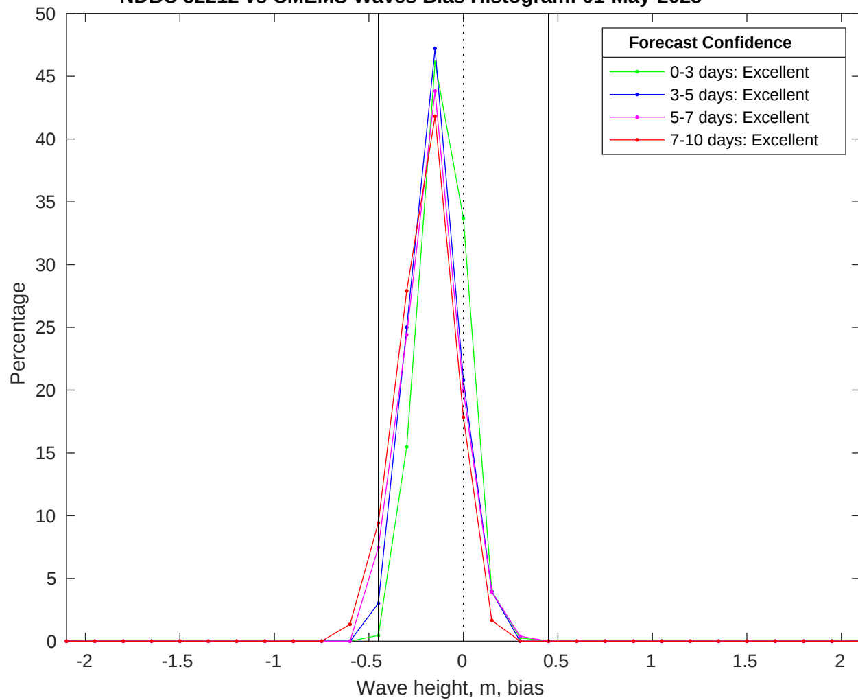
NDBC 52212 vs CMEMS Waves Bias Histogram: 01-May-2025
