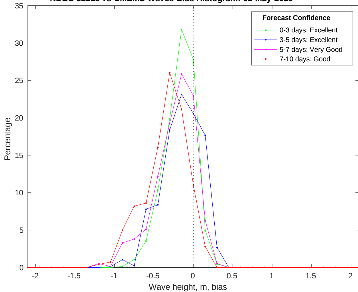
NDBC 52213 vs CMEMS Waves Bias Histogram: 01-May-2025
