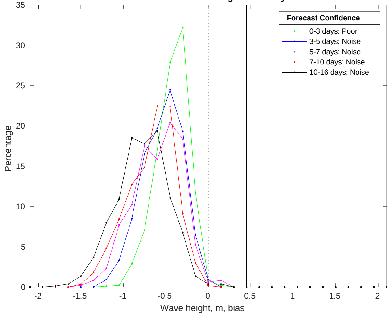
NDBC 52213 vs GFS Waves Bias Histogram: 01-May-2025
