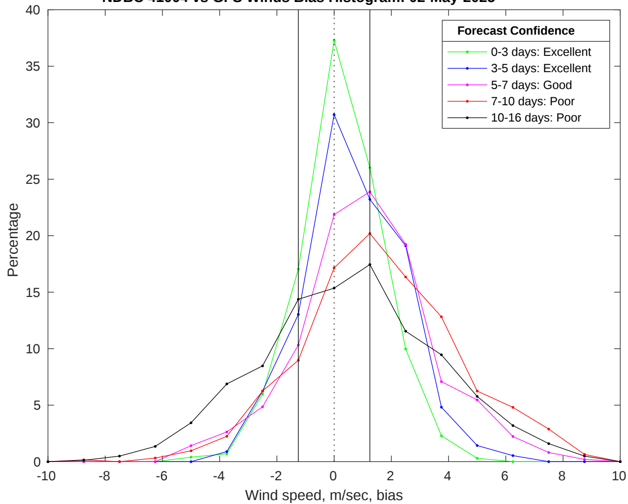
NDBC 41004 vs GFS Winds Bias Histogram: 02-May-2025
