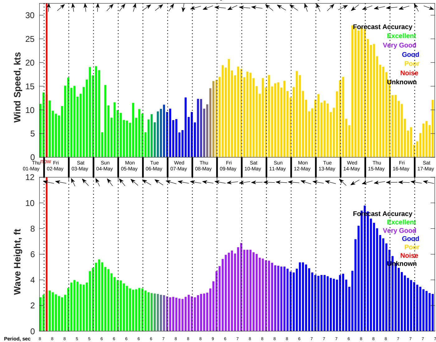
Wind & Wave Forecast for NDBC 41004 from 01-May-2025 19:00:00 to 17-May-2025 19:00:00
