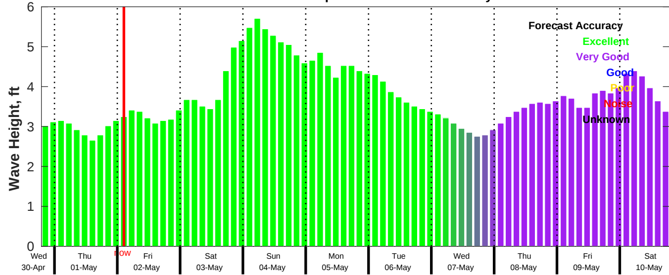
CMEMS Wave Forecast for NDBC 41013 from 30-Apr-2025 19:00:00 to 10-May-2025 19:00:00
