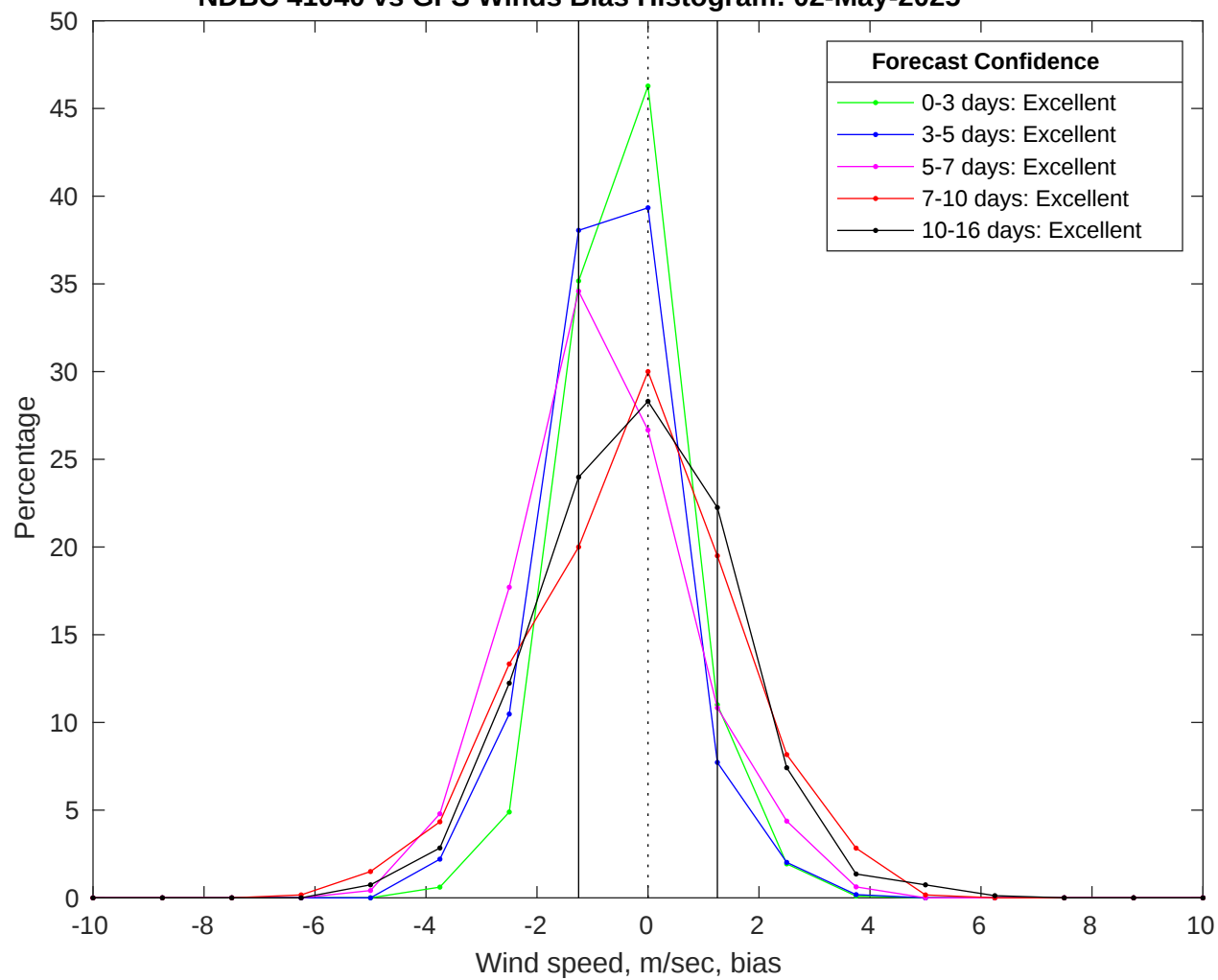
NDBC 41040 vs GFS Winds Bias Histogram: 02-May-2025
