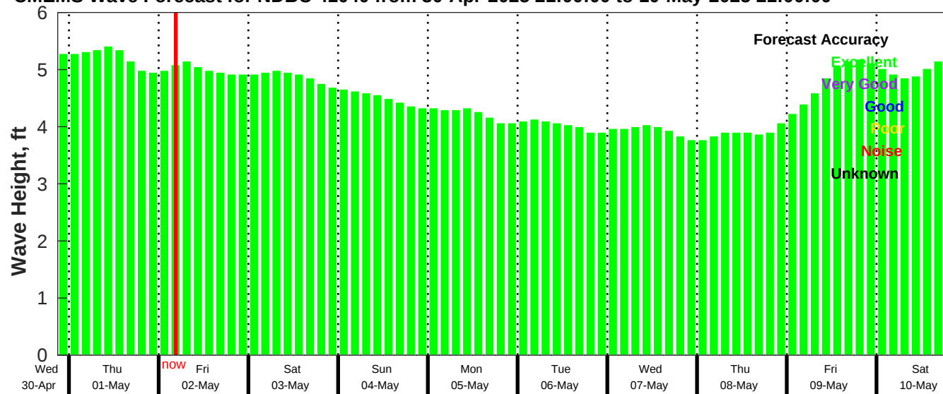
CMEMS Wave Forecast for NDBC 41040 from 30-Apr-2025 21:00:00 to 10-May-2025 21:00:00
