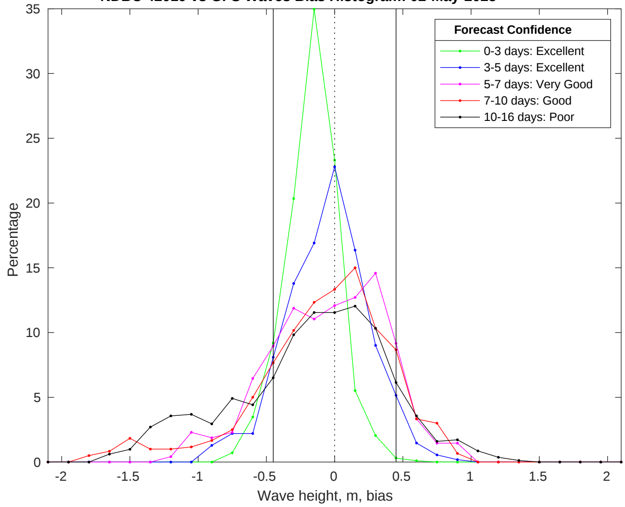
NDBC 42019 vs GFS Waves Bias Histogram: 02-May-2025
