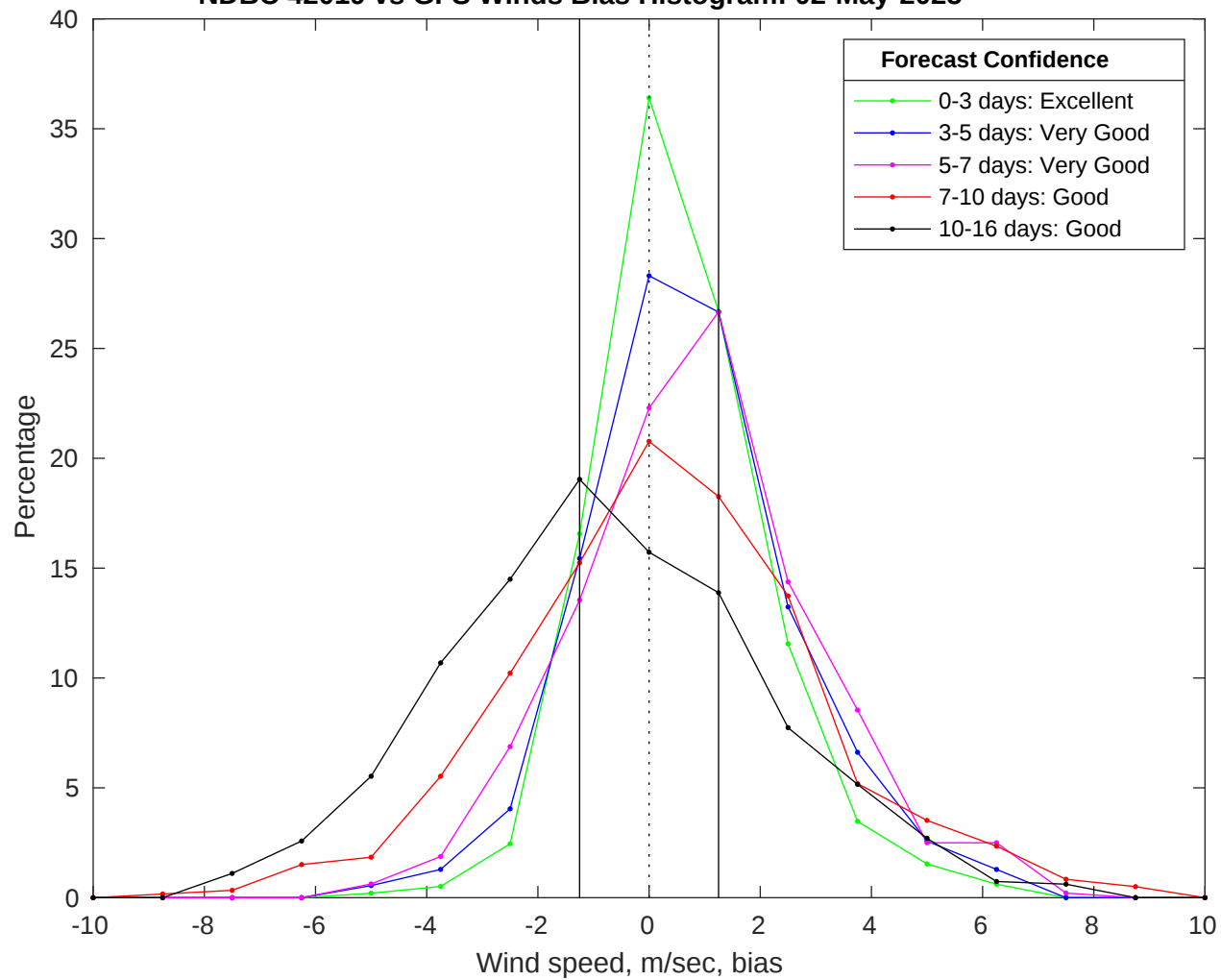
NDBC 42019 vs GFS Winds Bias Histogram: 02-May-2025
