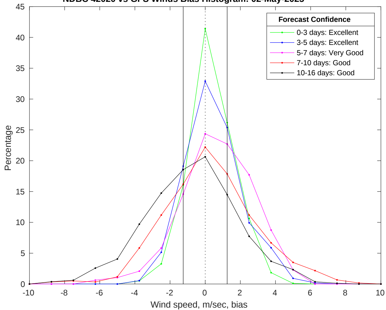
NDBC 42020 vs GFS Winds Bias Histogram: 02-May-2025
