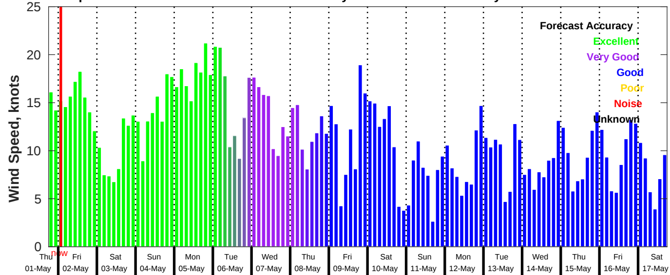
GFS Wind Speed Forecast for NDBC 42020 from 01-May-2025 18:00:00 to 17-May-2025 18:00:00
