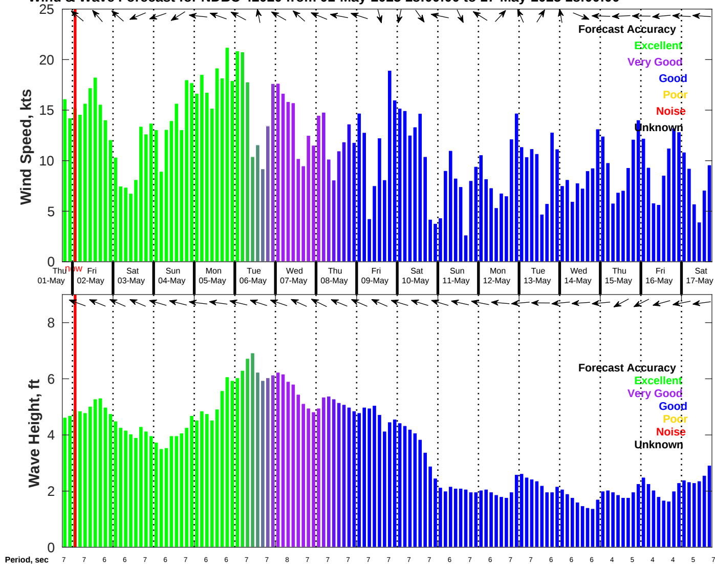
Wind & Wave Forecast for NDBC 42020 from 01-May-2025 18:00:00 to 17-May-2025 18:00:00
