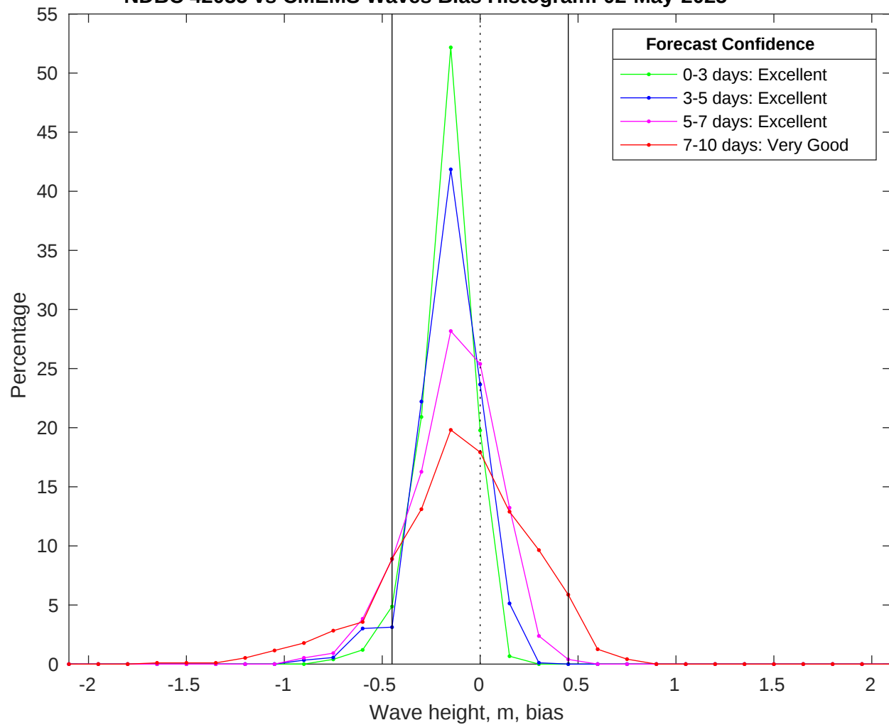
NDBC 42035 vs CMEMS Waves Bias Histogram: 02-May-2025
