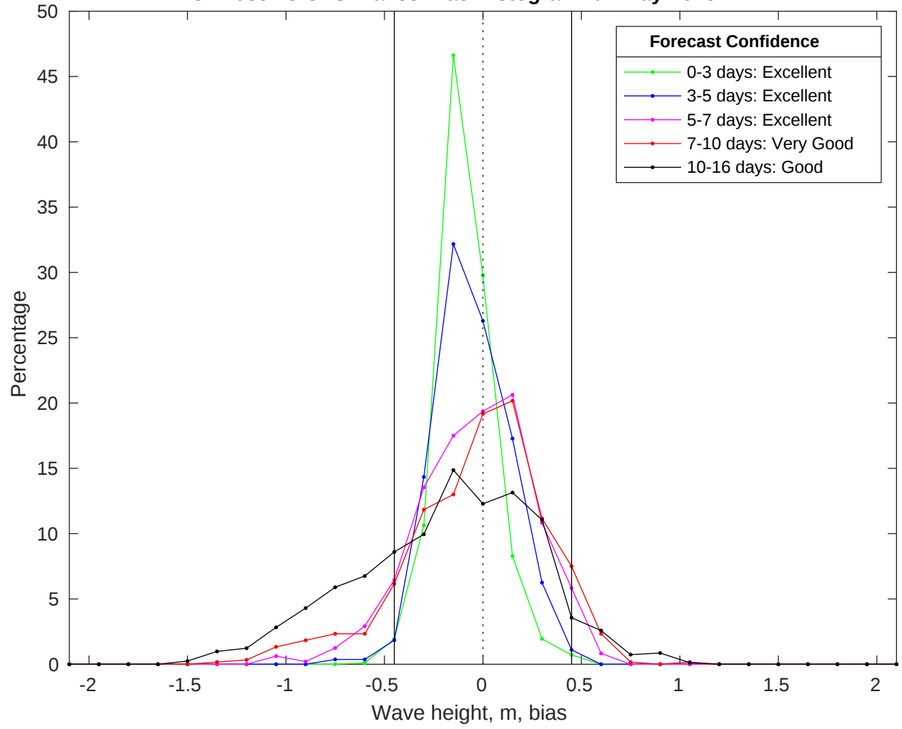
NDBC 42035 vs GFS Waves Bias Histogram: 02-May-2025
