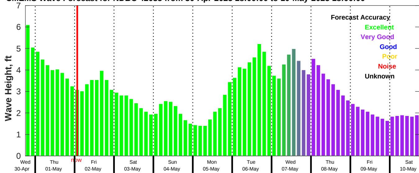
CMEMS Wave Forecast for NDBC 42035 from 30-Apr-2025 18:00:00 to 10-May-2025 18:00:00
