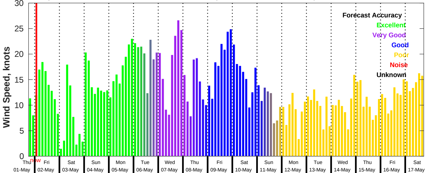
GFS Wind Speed Forecast for NDBC 42035 from 01-May-2025 18:00:00 to 17-May-2025 18:00:00
