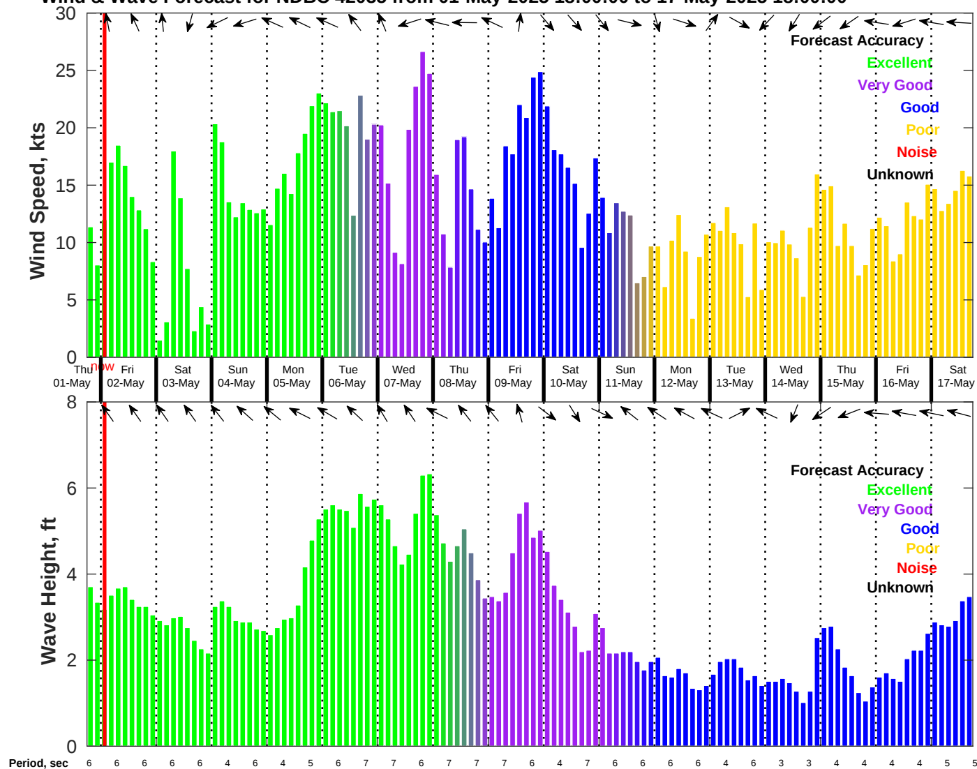
Wind & Wave Forecast for NDBC 42035 from 01-May-2025 18:00:00 to 17-May-2025 18:00:00
