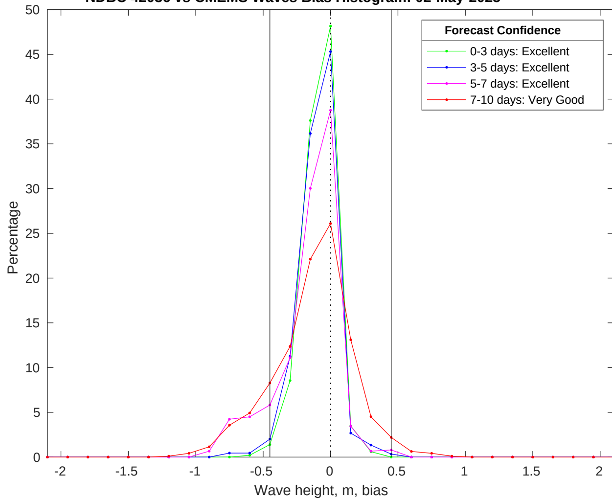
NDBC 42036 vs CMEMS Waves Bias Histogram: 02-May-2025
