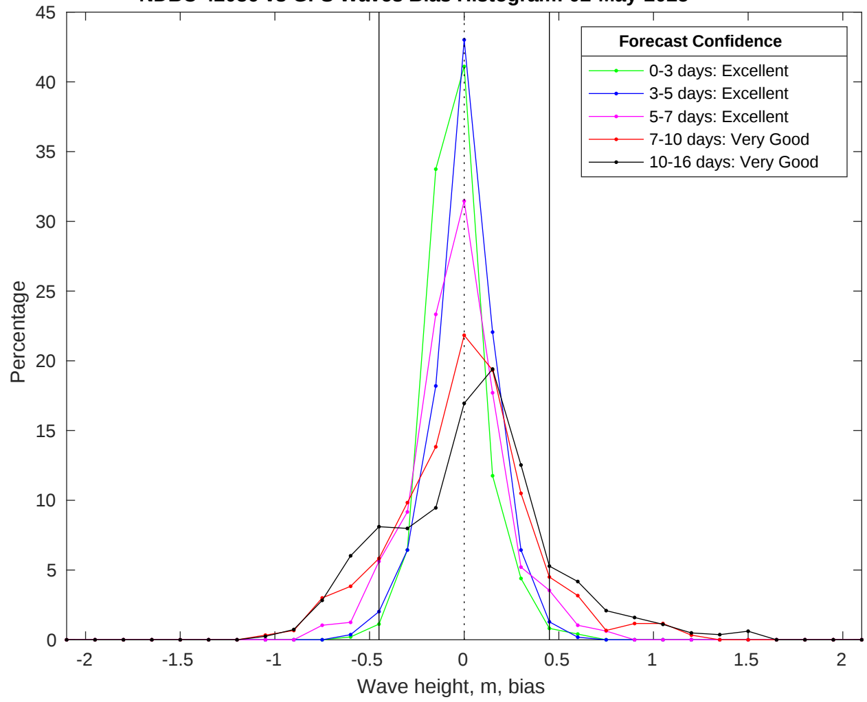
NDBC 42036 vs GFS Waves Bias Histogram: 02-May-2025
