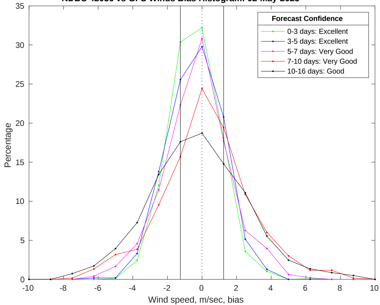
NDBC 42036 vs GFS Winds Bias Histogram: 02-May-2025
