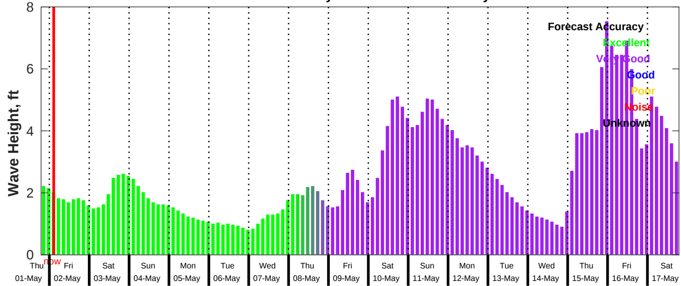
GFS Wave Forecast for NDBC 42036 from 01-May-2025 19:00:00 to 17-May-2025 19:00:00
