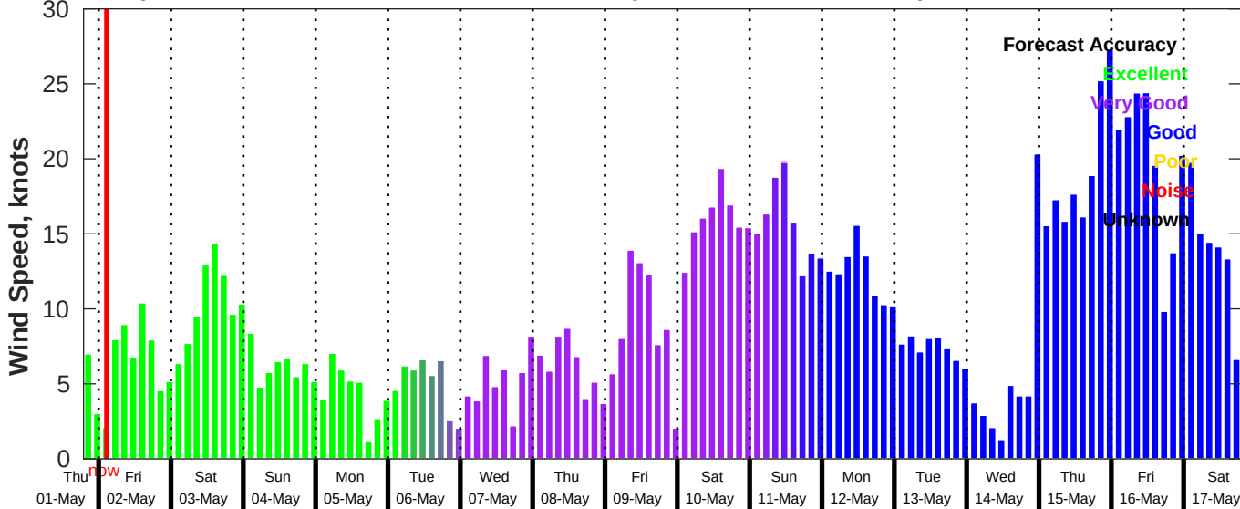
GFS Wind Speed Forecast for NDBC 42036 from 01-May-2025 19:00:00 to 17-May-2025 19:00:00
