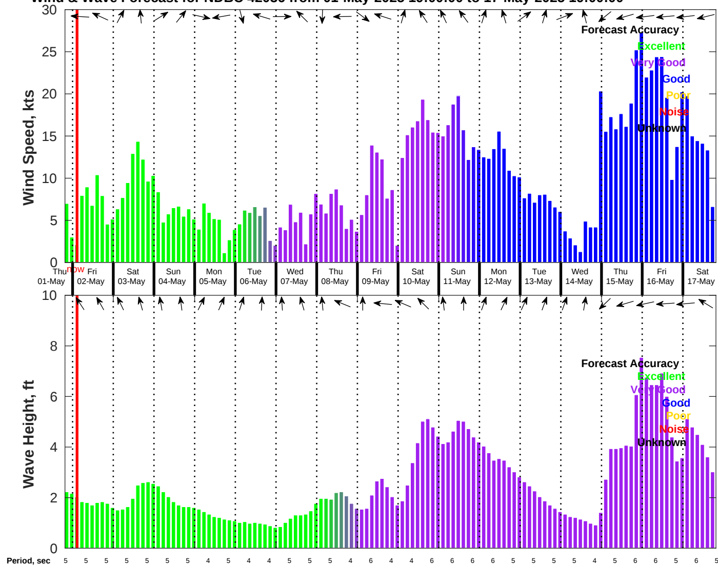
Wind & Wave Forecast for NDBC 42036 from 01-May-2025 19:00:00 to 17-May-2025 19:00:00
