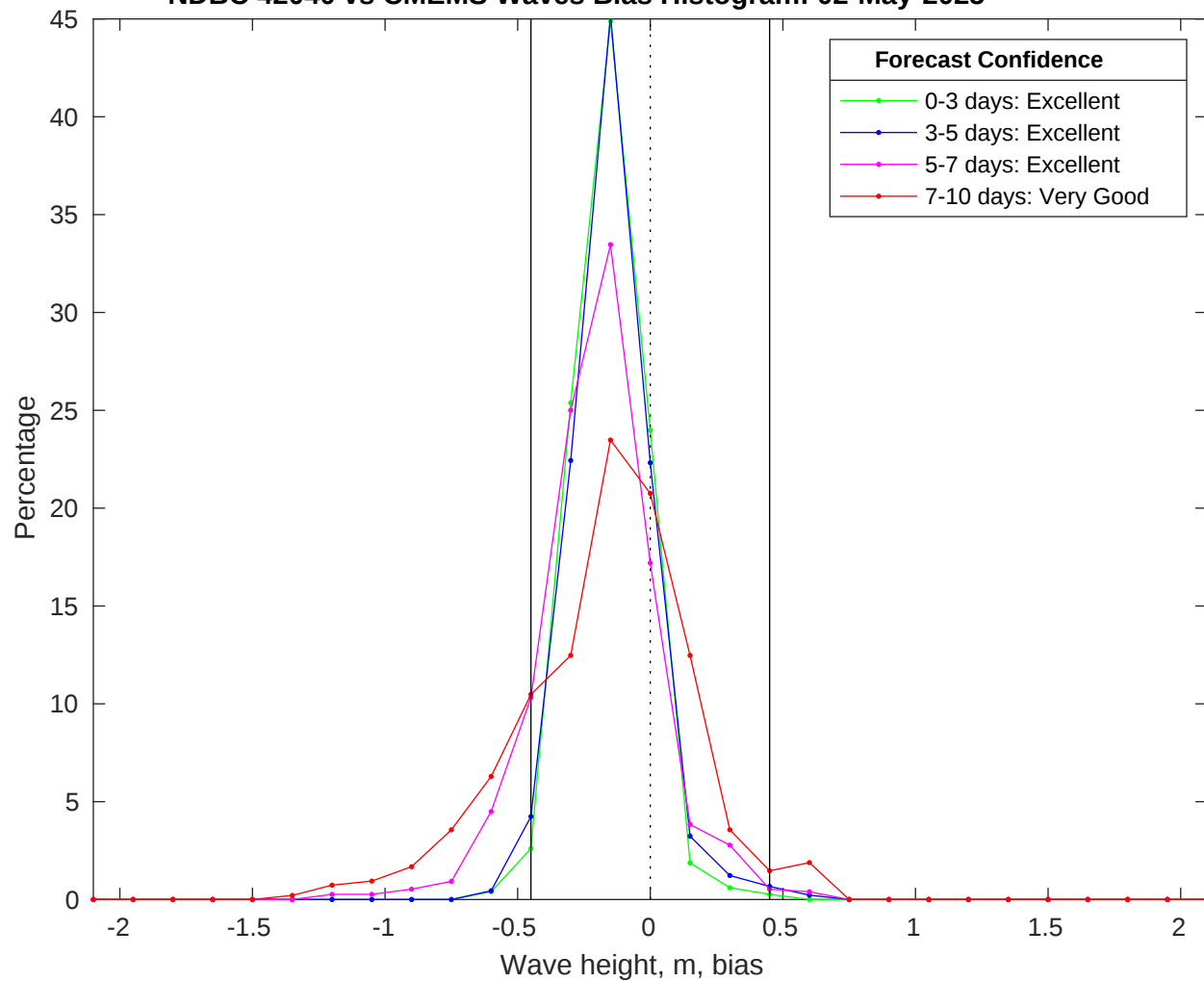
NDBC 42040 vs CMEMS Waves Bias Histogram: 02-May-2025
