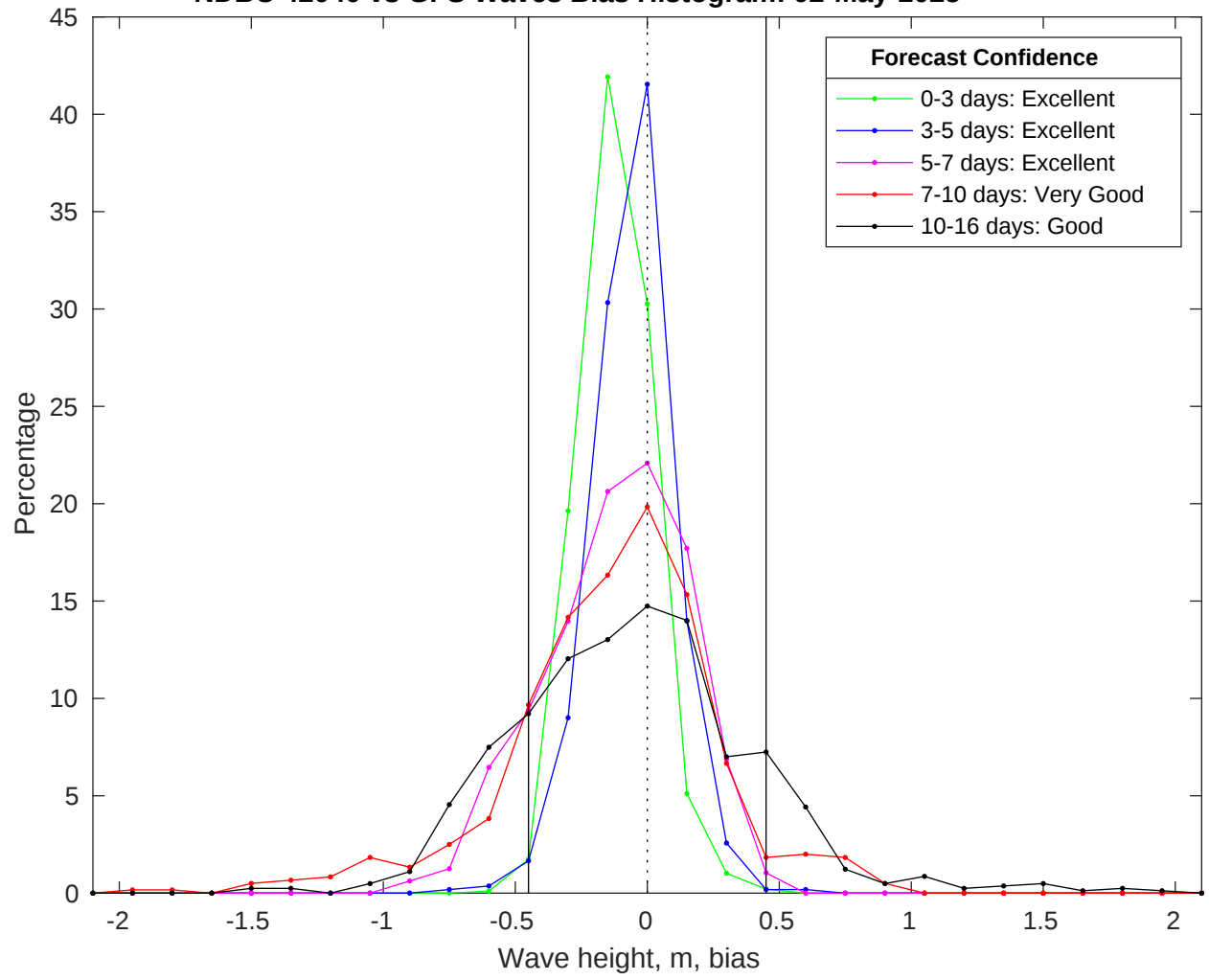
NDBC 42040 vs GFS Waves Bias Histogram: 02-May-2025
