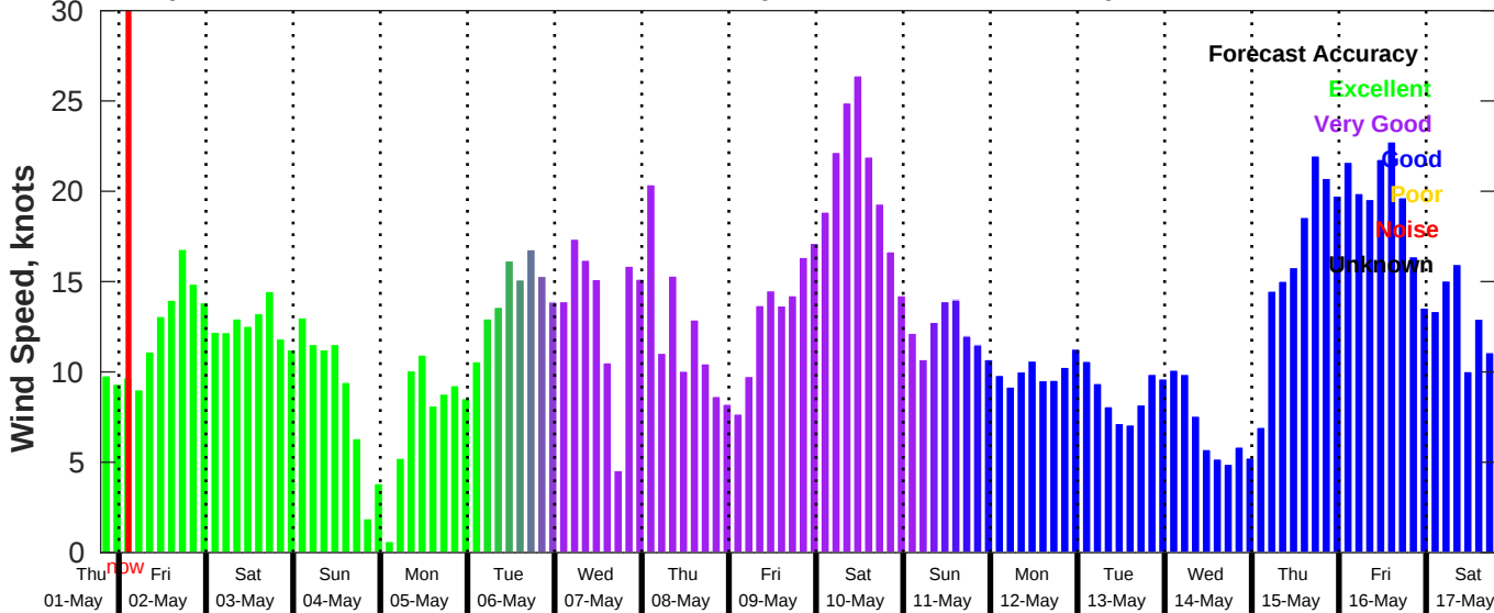
GFS Wind Speed Forecast for NDBC 42040 from 01-May-2025 19:00:00 to 17-May-2025 19:00:00
