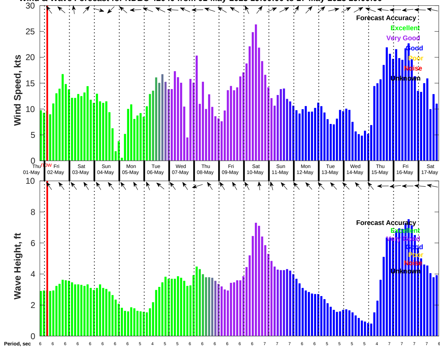
Wind & Wave Forecast for NDBC 42040 from 01-May-2025 19:00:00 to 17-May-2025 19:00:00
