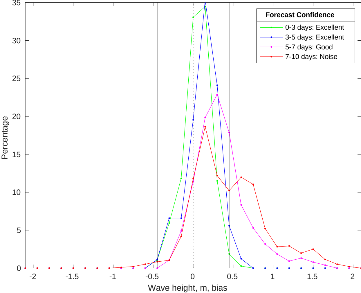
NDBC 46011 vs CMEMS Waves Bias Histogram: 02-May-2025
