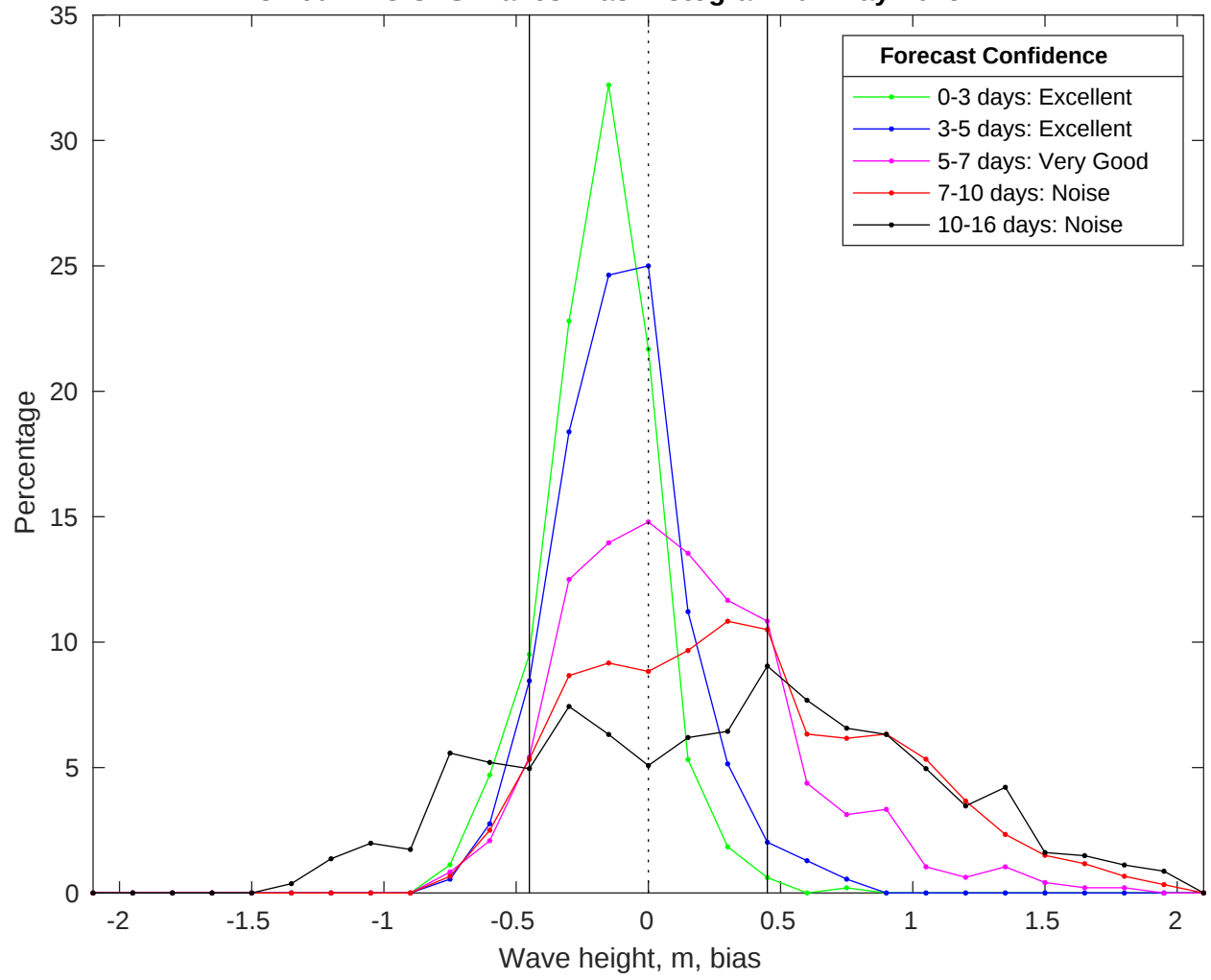
NDBC 46011 vs GFS Waves Bias Histogram: 02-May-2025
