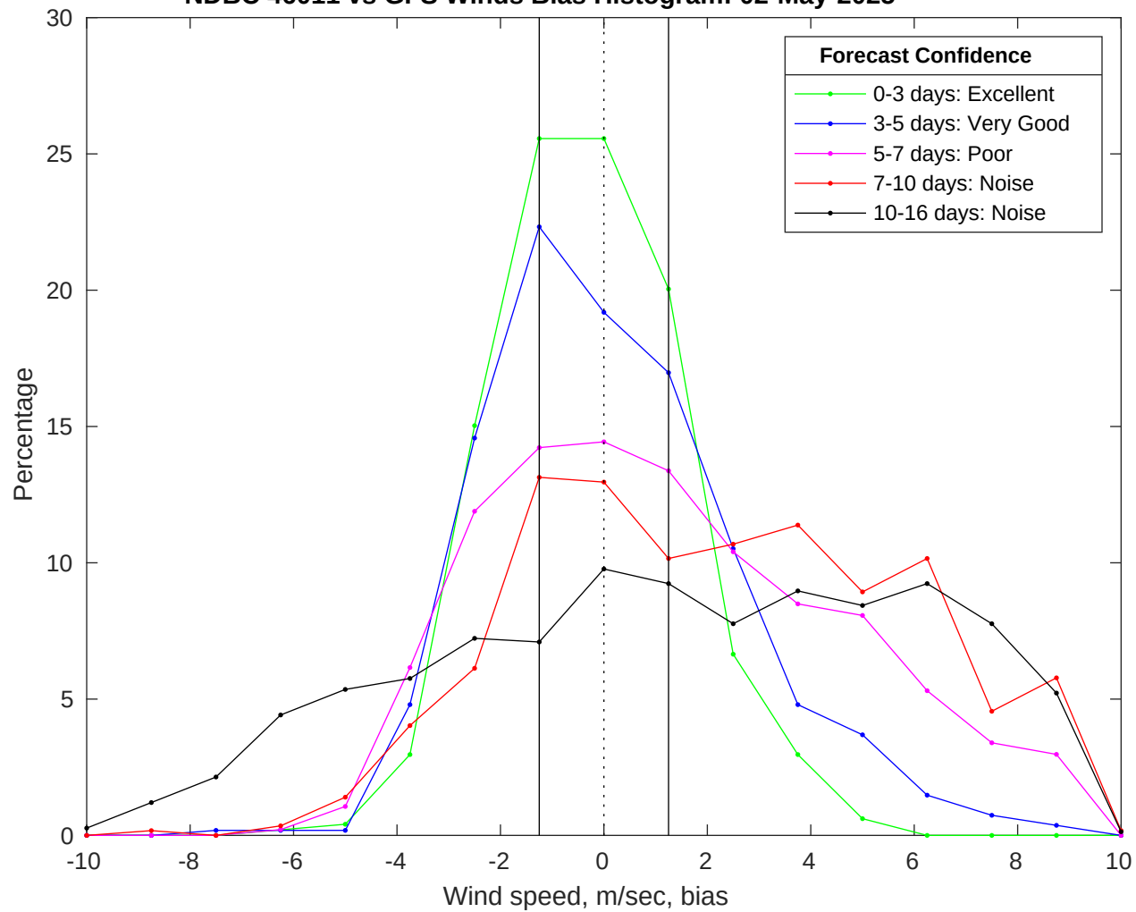
NDBC 46011 vs GFS Winds Bias Histogram: 02-May-2025
