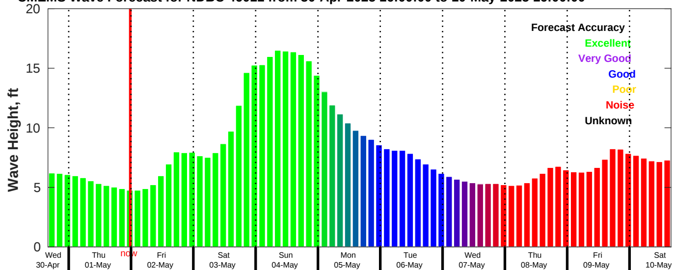
CMEMS Wave Forecast for NDBC 46011 from 30-Apr-2025 16:00:00 to 10-May-2025 16:00:00
