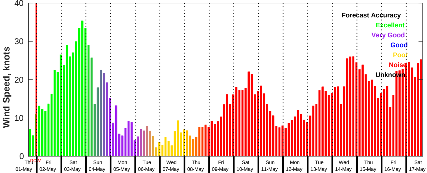
GFS Wind Speed Forecast for NDBC 46011 from 01-May-2025 16:00:00 to 17-May-2025 16:00:00
