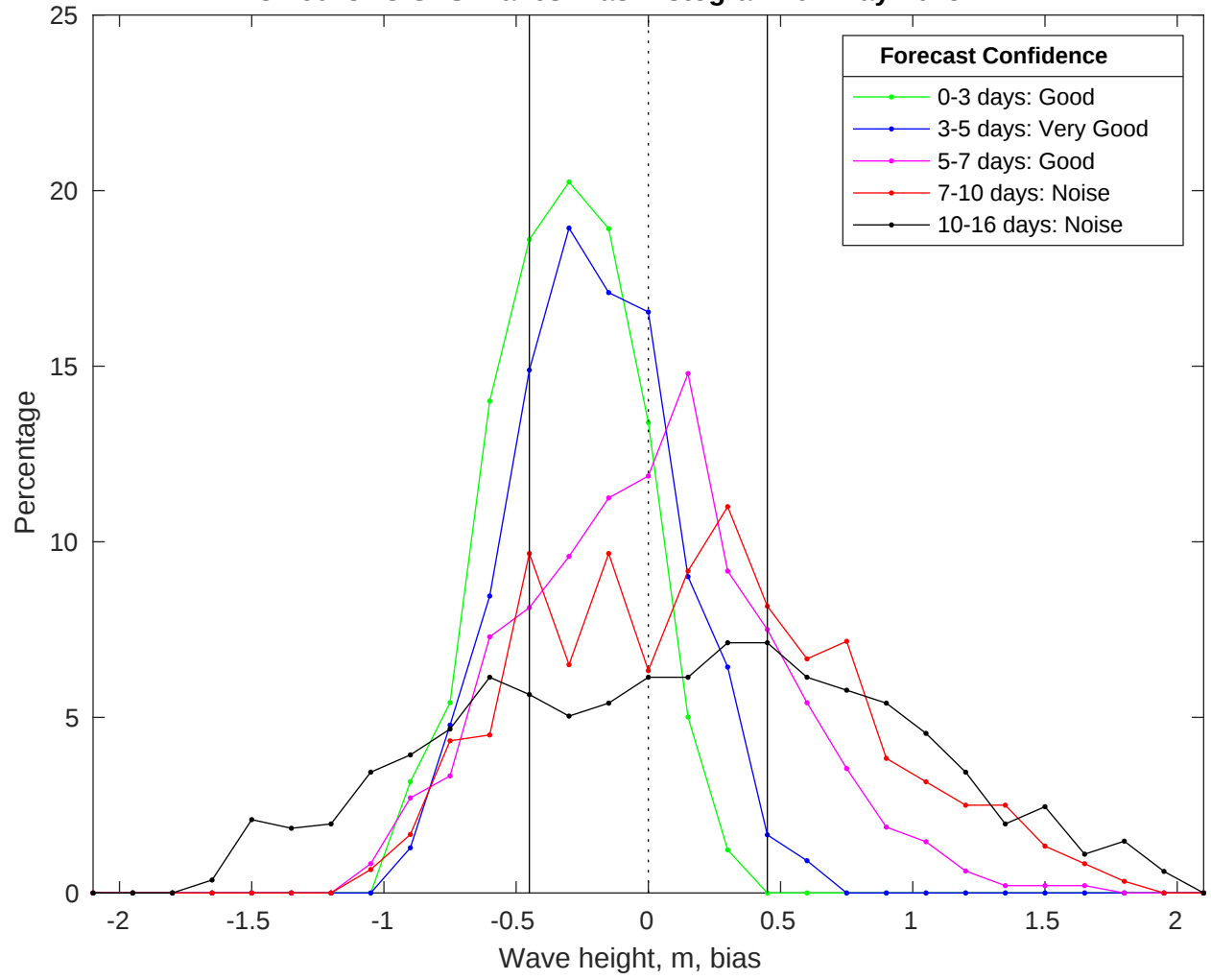
NDBC 46028 vs GFS Waves Bias Histogram: 02-May-2025
