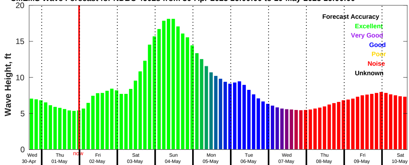
CMEMS Wave Forecast for NDBC 46028 from 30-Apr-2025 16:00:00 to 10-May-2025 16:00:00
